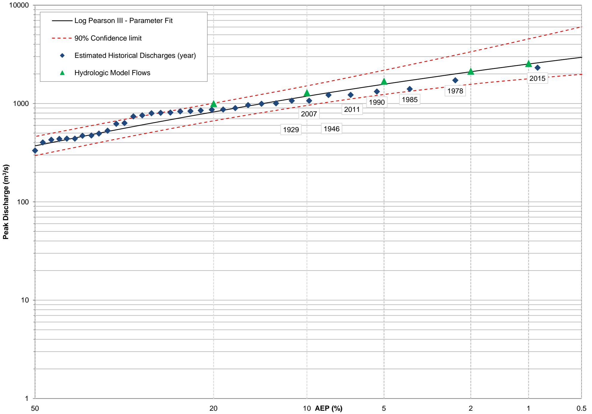
FIGURE 39 PATERSON RIVER GOSTWYCK - 210079 FFA - LP3 DISTRIBUTION
