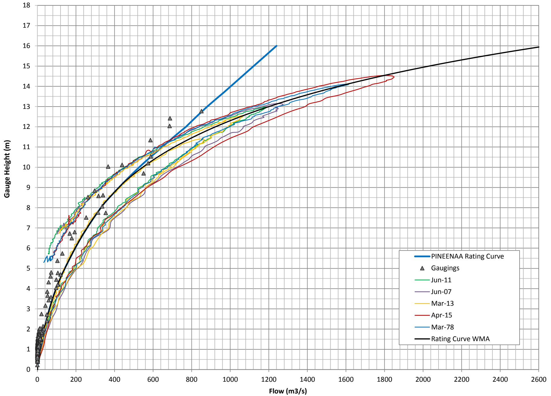
PATERSON RIVER GOSTWYCK PINEENA - 210079 REVISED RATING CURVE AND GAUGINGS
