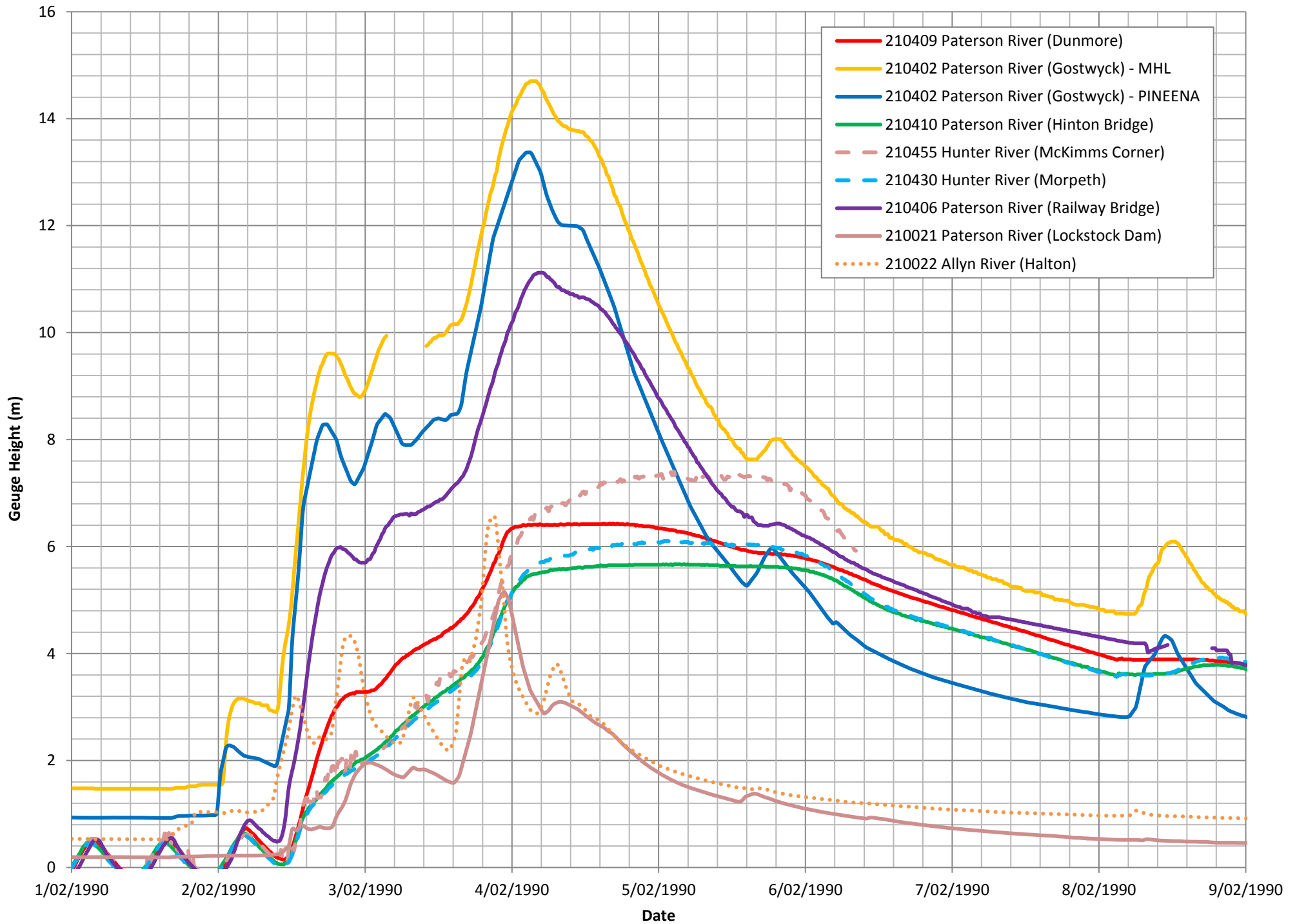
FIGURE 12 WATER LEVEL DATA FEBRUARY 1990 EVENT
