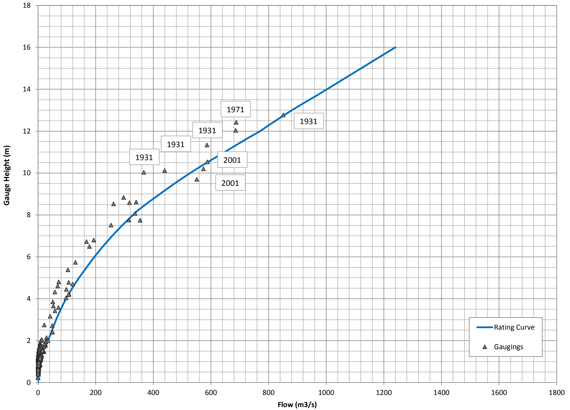
FIGURE 8 PATERSON RIVER GOSTWYCK PINEENA - 2100079 RATING CURVE AND GAUGINGS
