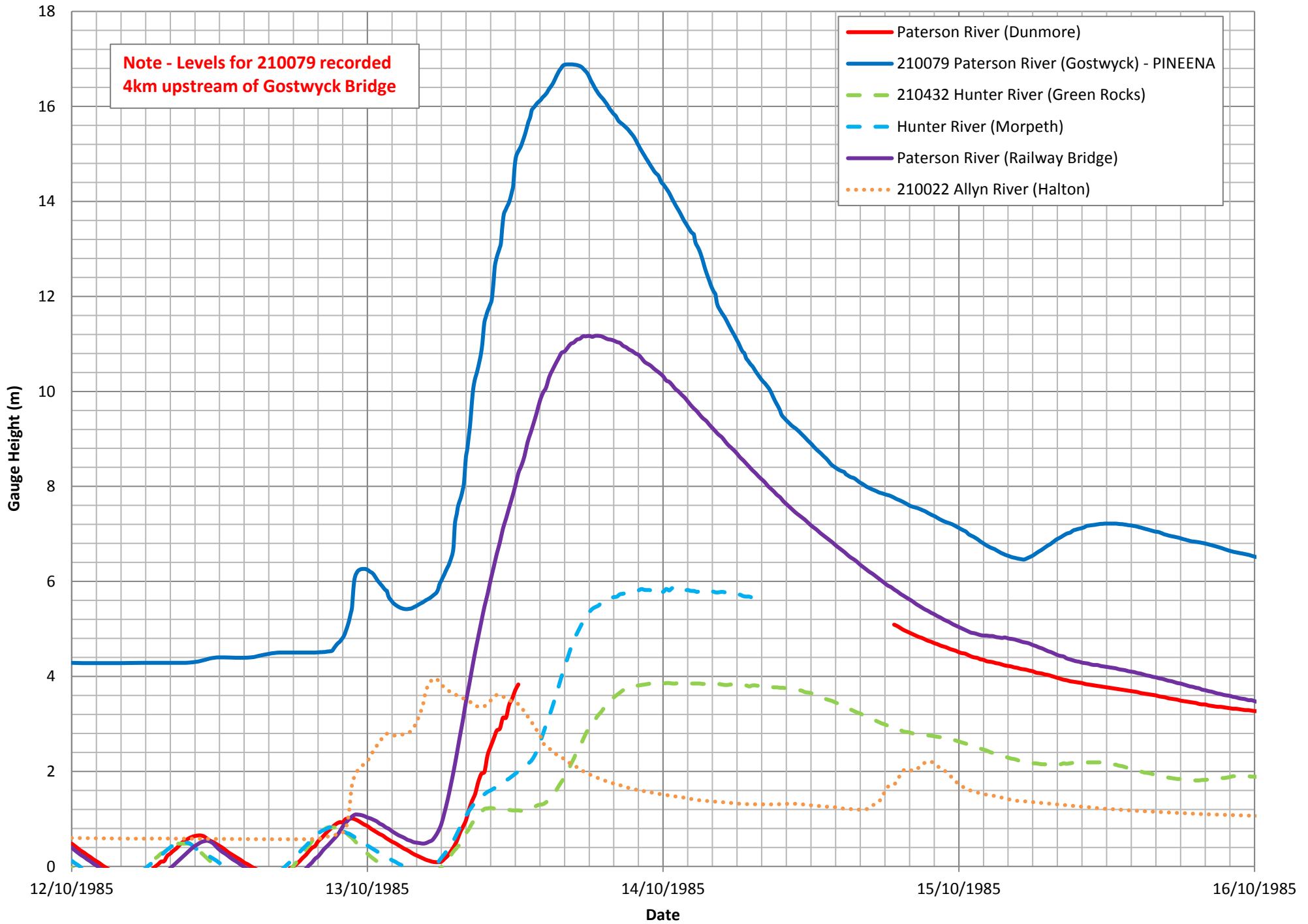
FIGURE 11 WATER LEVEL DATA OCTOBER 1985 EVENT
