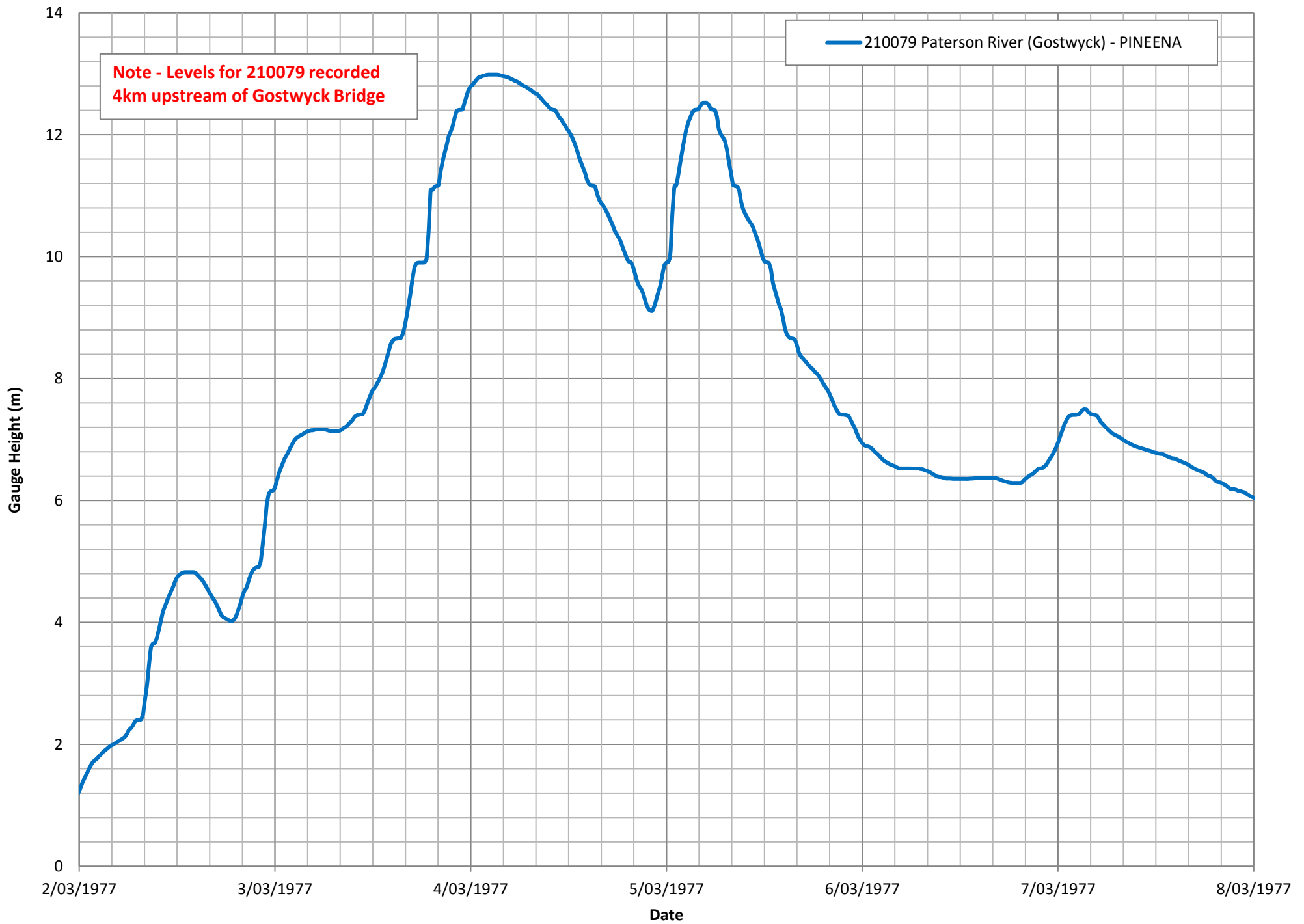
FIGURE 9 WATER LEVEL DATA MARCH 1977 EVENT
