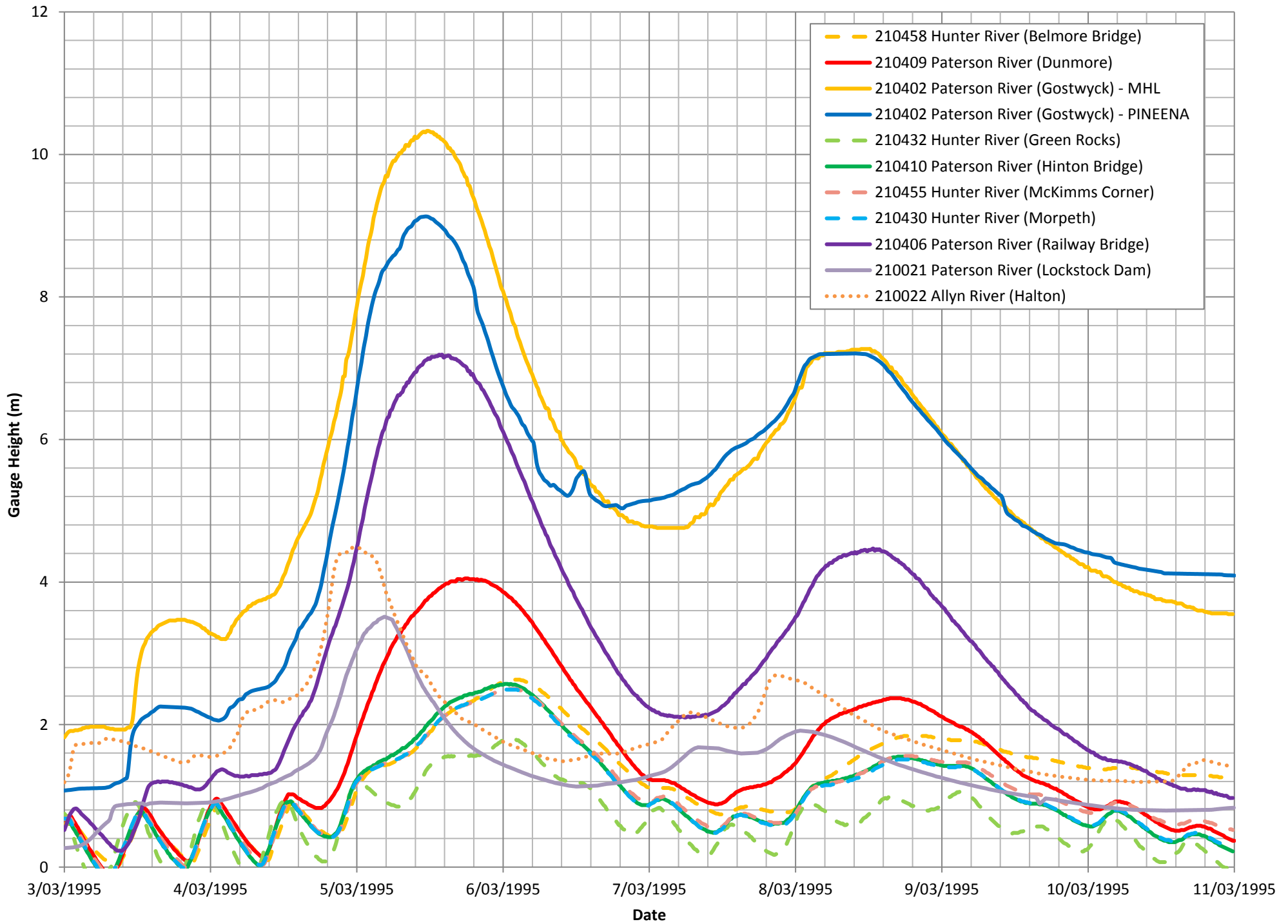
FIGURE 13 WATER LEVEL DATA MARCH 1995 EVENT
