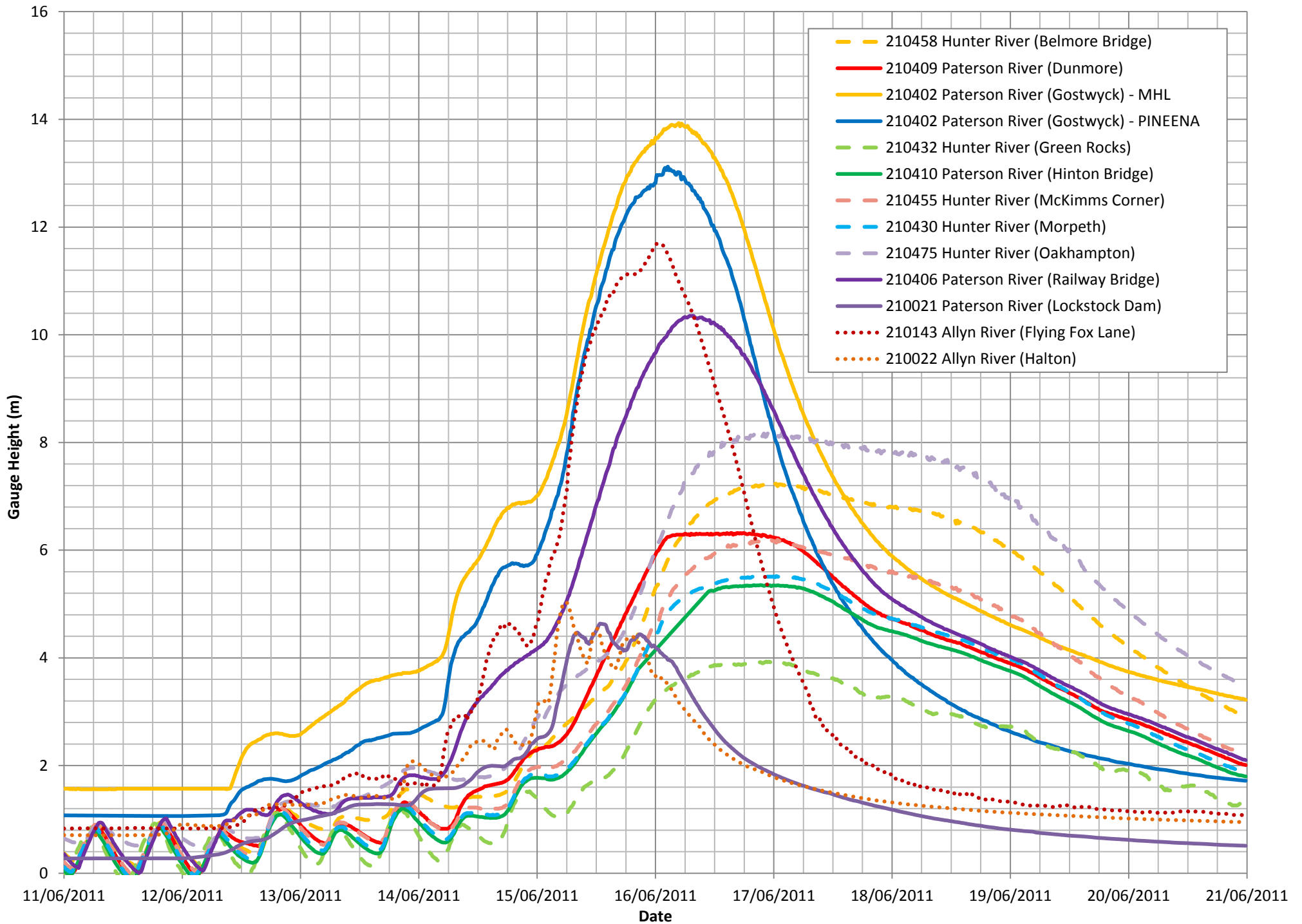
FIGURE 16 WATER LEVEL DATA JUNE 2011 EVENT
