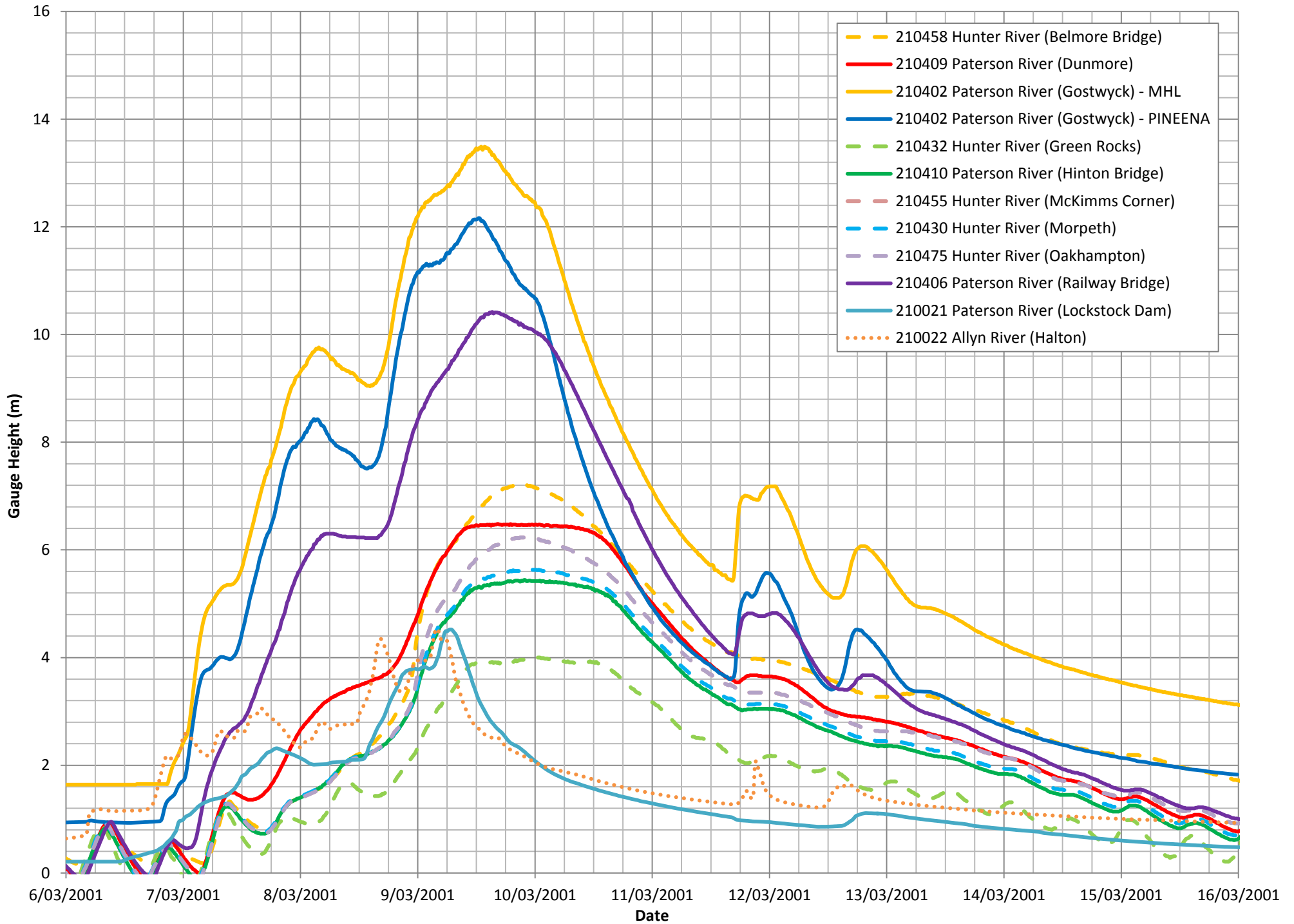
FIGURE 14 WATER LEVEL DATA MARCH 2001 EVENT
