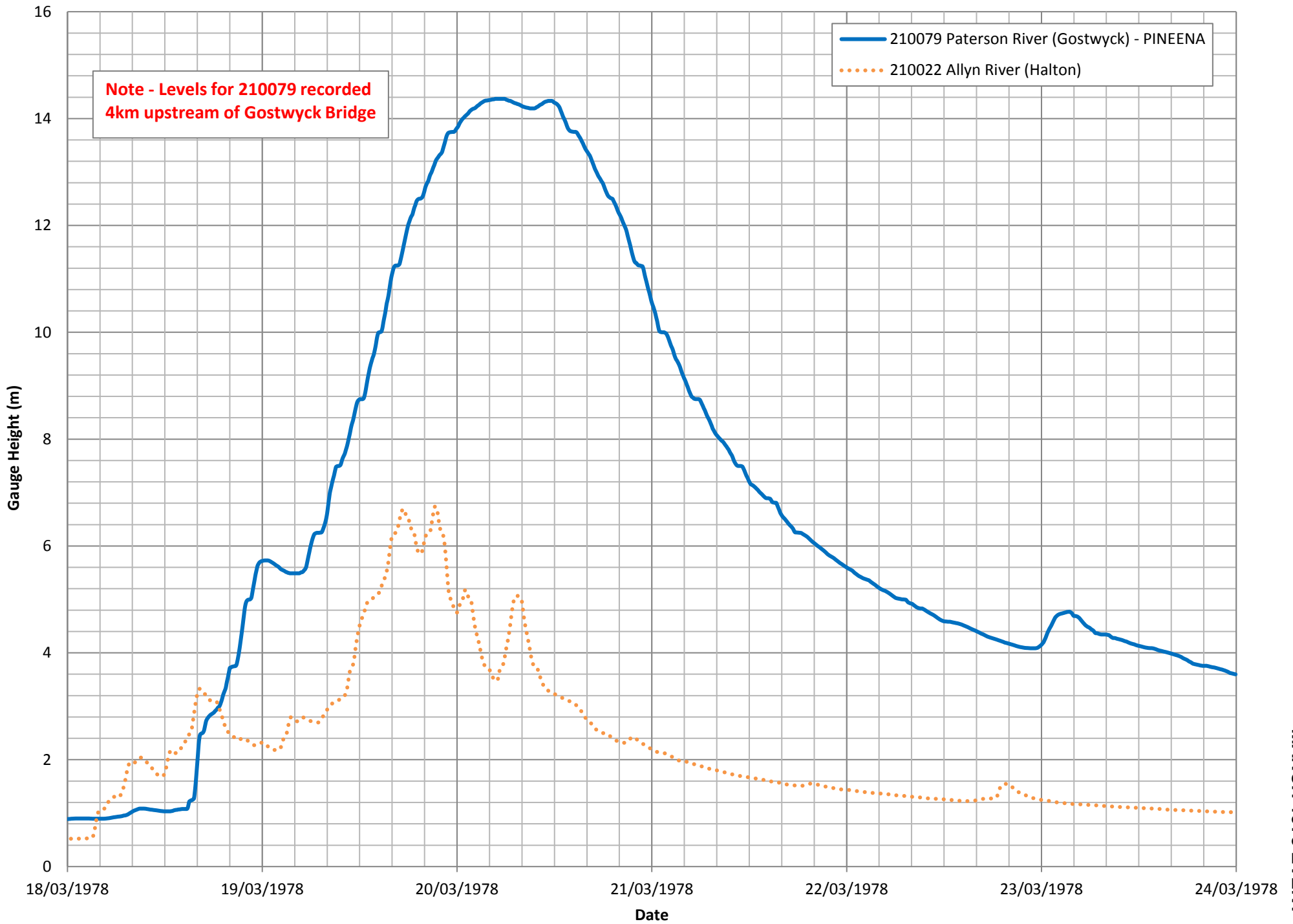
FIGURE 10 WATER LEVEL DATA MARCH 1978 EVENT
