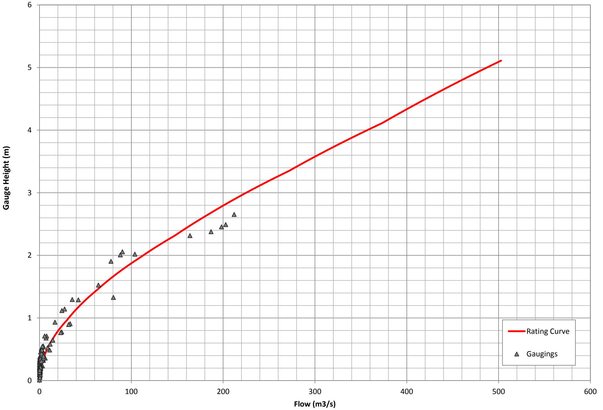
FIGURE 6 PATERSON RIVER AT LOSTOCK DAM- 210021 RATING CURVE AND GAUGINGS
