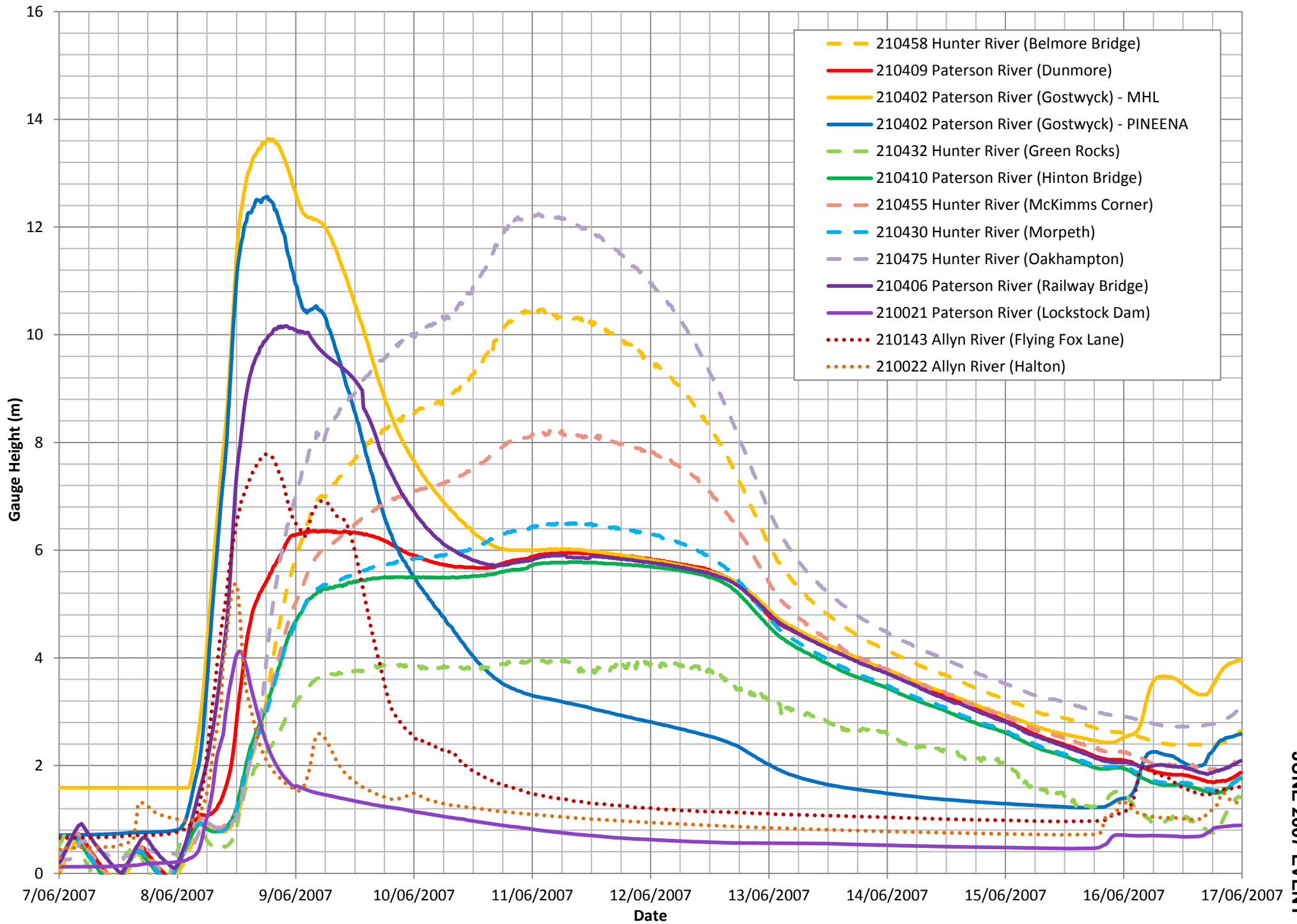
FIGURE 15 WATER LEVEL DATA JUNE 2007 EVENT
