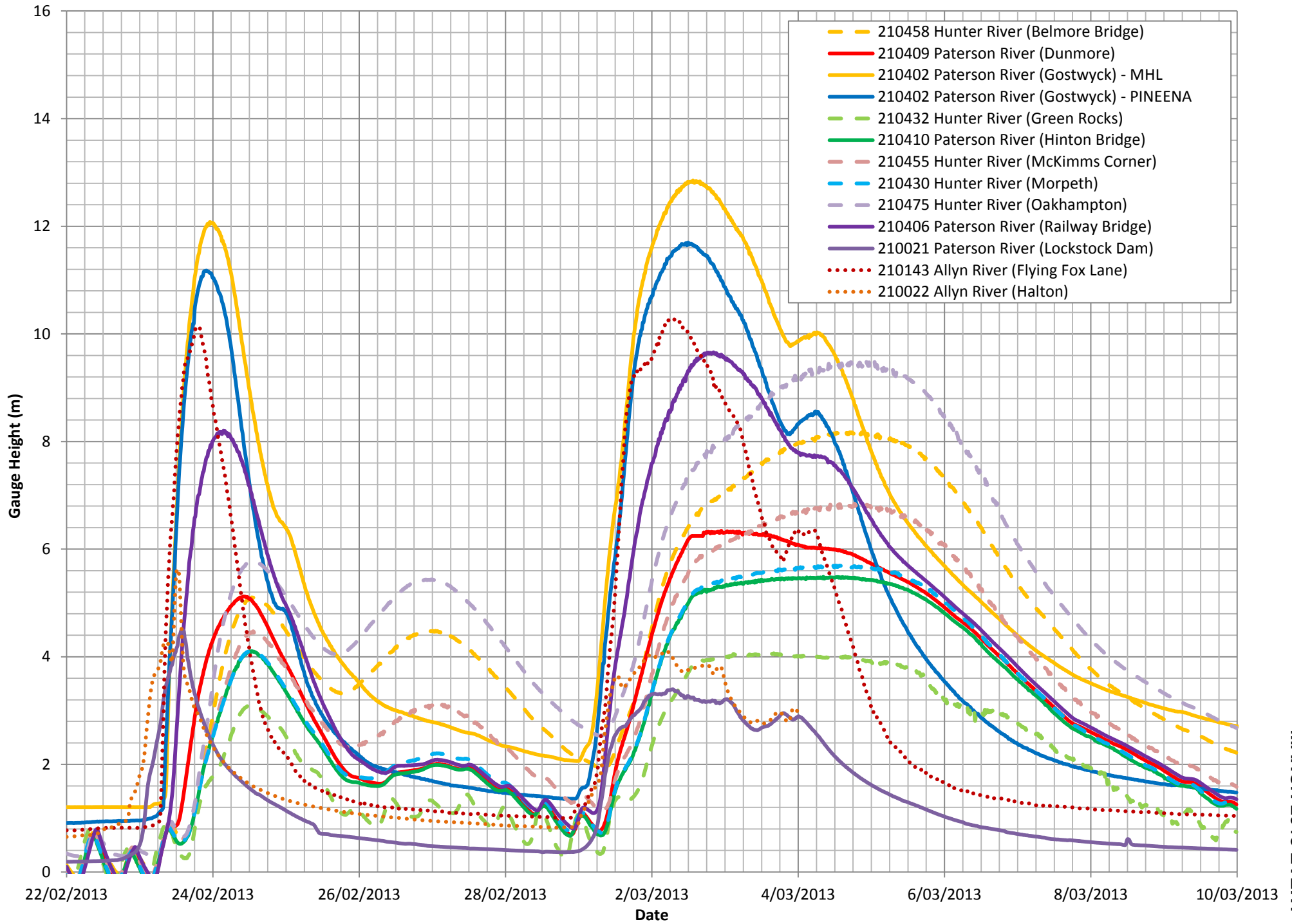
FIGURE 17 WATER LEVEL DATA MARCH 2013 EVENT
