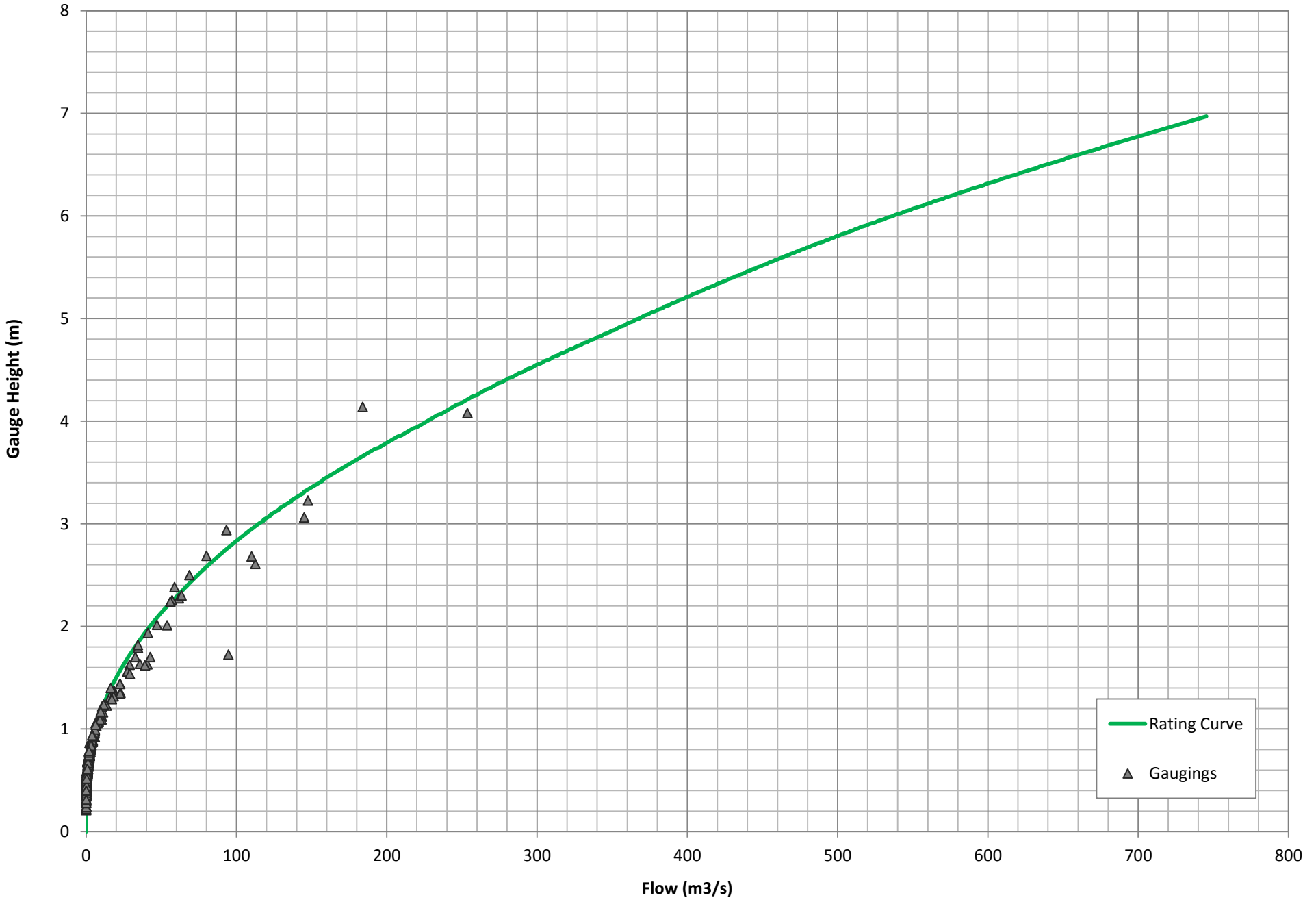
FIGURE 5 ALLYN RIVER HALTON - 210022 RATING CURVE AND GAUGINGS
