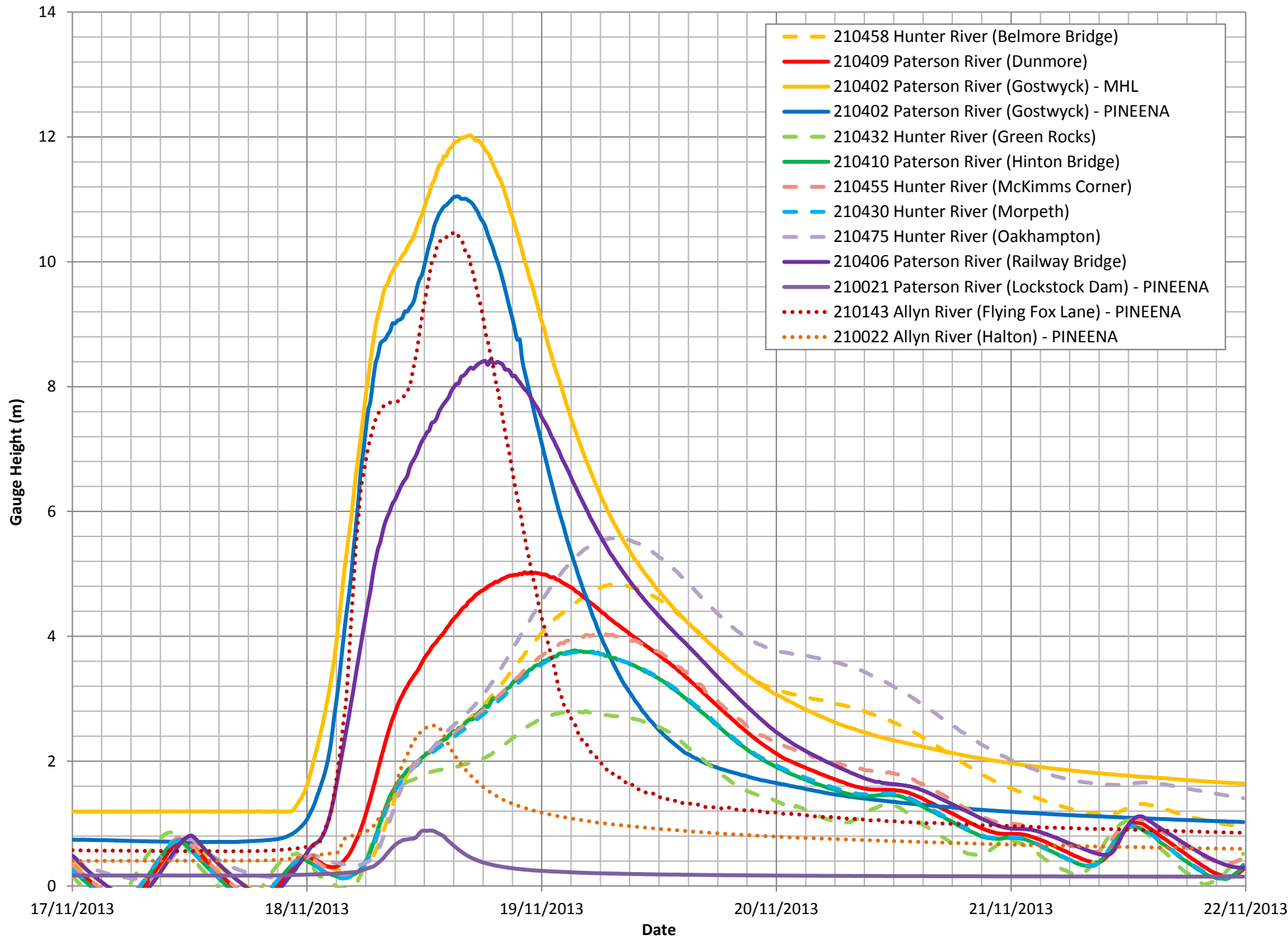
FIGURE 18 WATER LEVEL DATA NOVEMBER 2013 EVENT
