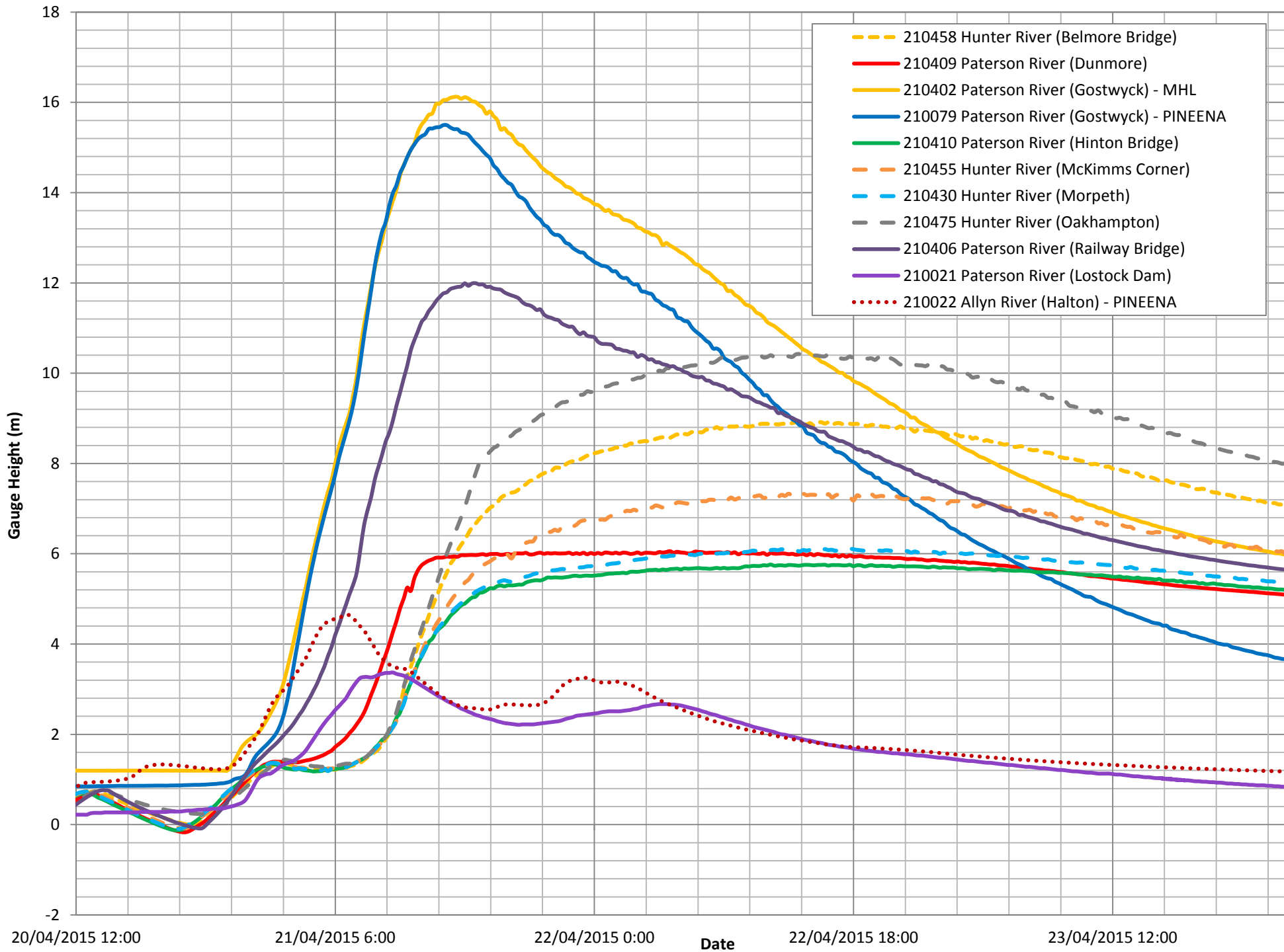
FIGURE 19 WATER LEVEL DATA APRIL 2015 EVENT
