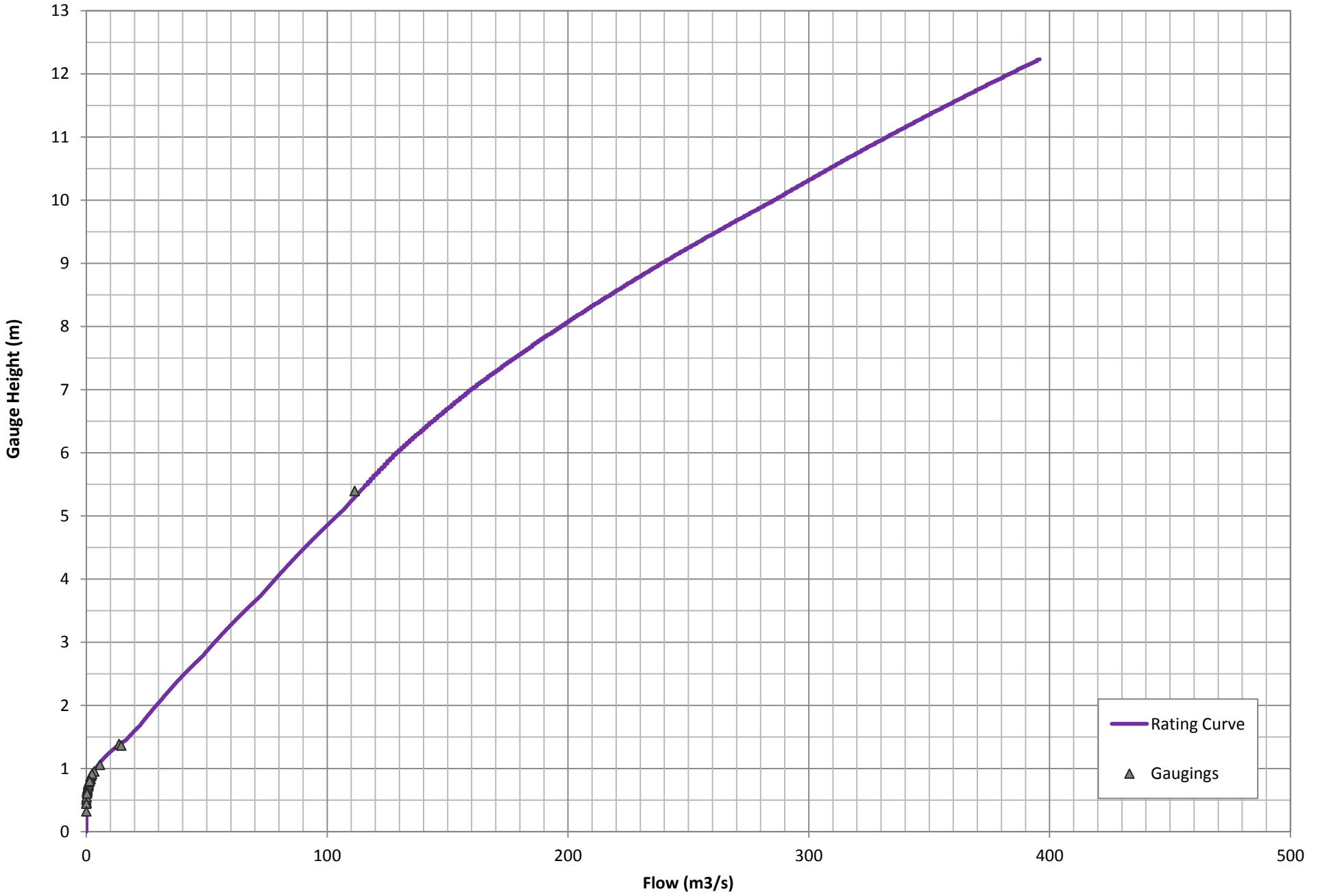
FIGURE 7 ALLYN RIVER FLYING FOX LANE - 210043 RATING CURVE AND GAUGINGS
